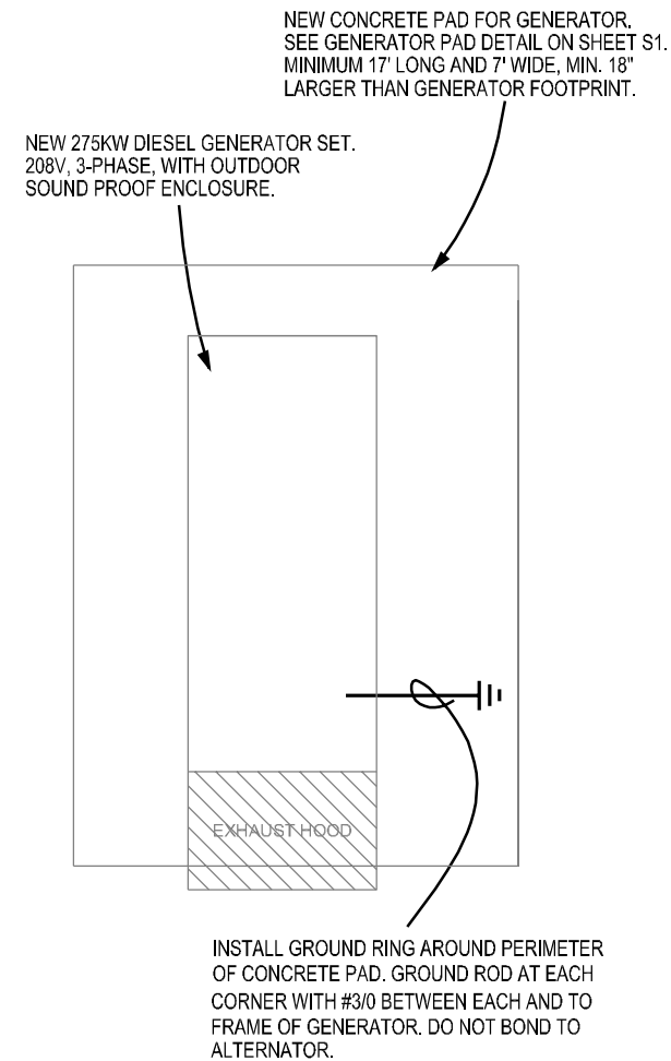
2 E2 GENERATOR PAD DETAIL NO SCALE
